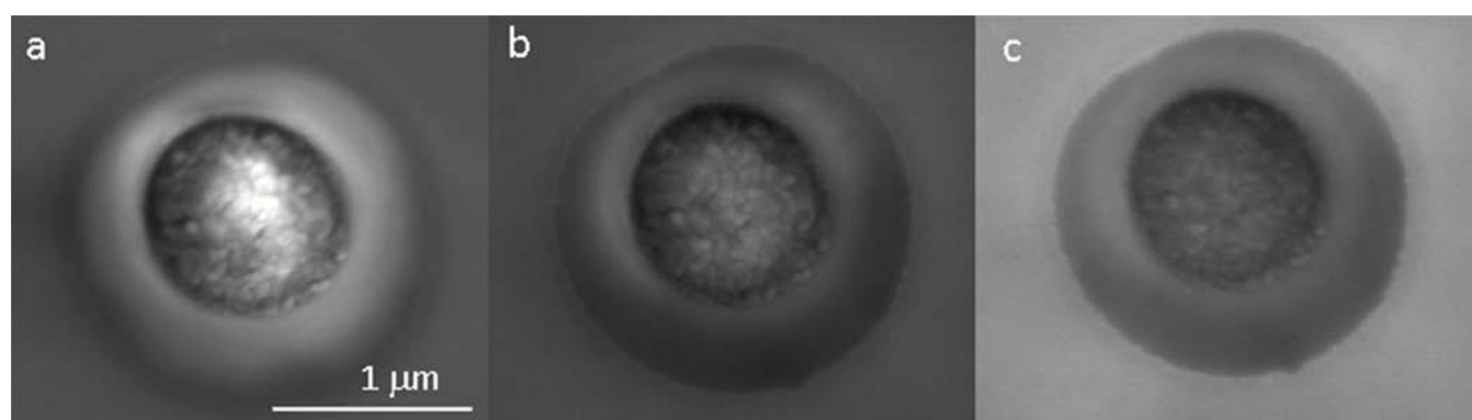
Figure 1. Liquid SEM SE imaging of boehmite particles in DI water: (a) 5 kV; (b) 8 kV; and (c) 10 kV.
