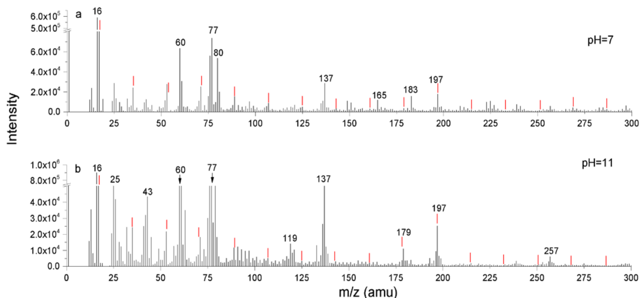
Figure 2. Negative m/z spectra of synthesized boehmite particles in DI water by ToF-SIMS: (a) natural pH and (b) alkaline pH. Red bars indicate locations of water clusters.
