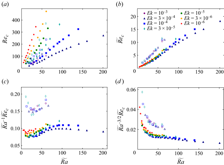
Figure 2. Reynolds number characterising the flow speeds of the fluctuating (convective) velocity versus the reduced Rayleigh number, \tilde{Ra} : (a) the convective Reynolds number Re_c ; (b) the rescaled convective Reynolds number \tilde{Re}_c = Ek^{1/3} Re_c ; (c) the compensated convective Reynolds number \tilde{Re}_c \tilde{Ra}^{-1} ; (d) the compensated convective Reynolds number \tilde{Re}_c \tilde{Ra}^{-3/2} . The filled symbols represent \eta = 0.35 cases and the hollow symbols represent \eta = 0.7 cases.
