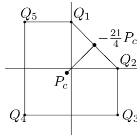
FIGURE 2. \text{Bl}_{p,q}\mathbb{P}^2 .
