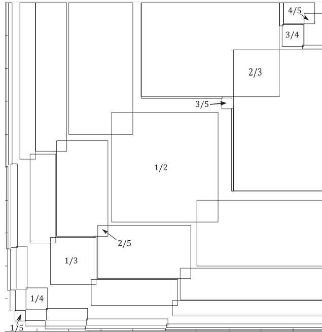
FIGURE 5. The rotation number diagram for the model map with k = 2 , reparameterized for clarity.
