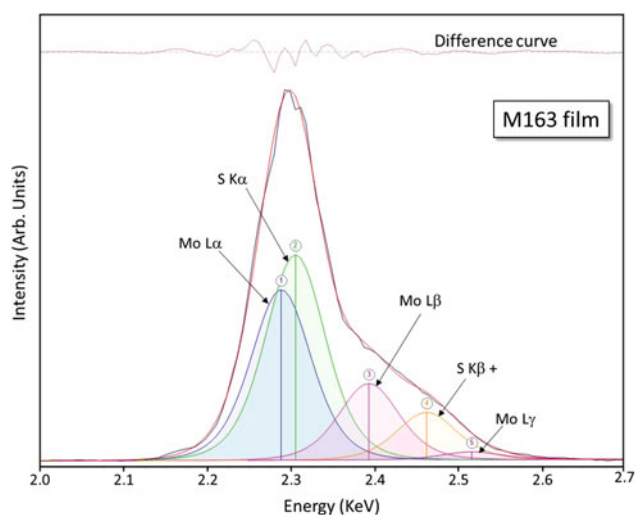
Figure 8. Resulting fit of emission lines for Mo L and S K-series peaks. This model, outlined in the text, establishes the ability to extract the intensity for the Mo L\alpha and S K\alpha peaks for means of quantifying film composition.
