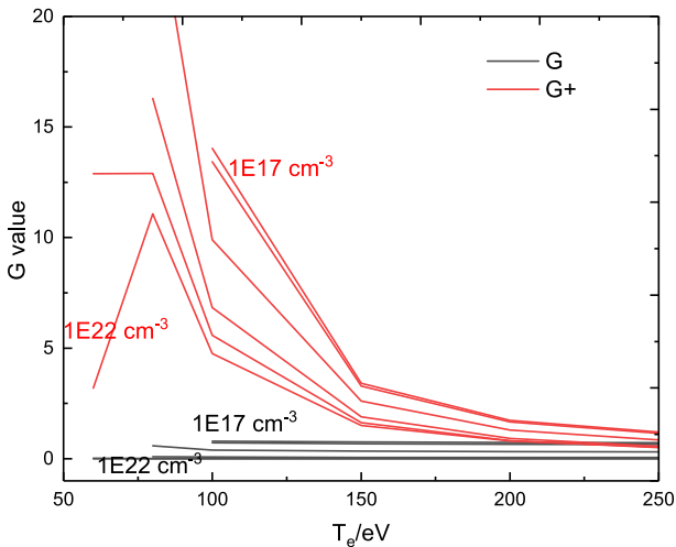
Figure 6. The G+ and G values. Every line has same electron density, which spans from 10 17 cm -3 to 10 22 cm -3 exponentially, and the line ratios are plotted as a function of electron temperature.
