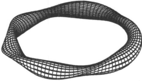
Three-dimensional picture of a flux surface of an l = 2 stellarator. The elliptical cross section rotates poloidally when traversing toroidally.
