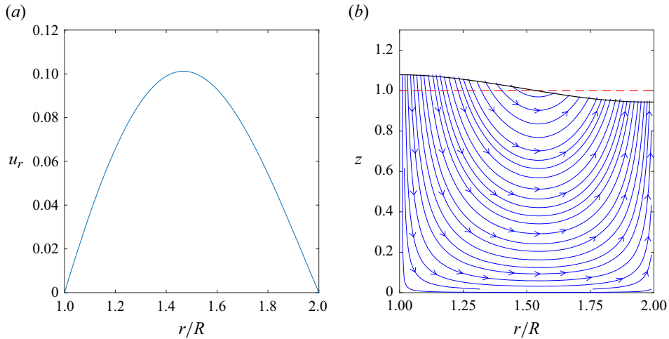
Figure 4. (a) Leading eigenfunction u_r = Y_1(\alpha\sqrt{\Lambda})J_1(r\sqrt{\Lambda}) - J_1(\alpha\sqrt{\Lambda})Y_1(r\sqrt{\Lambda}) of the radial perturbation mode for the same parameters as in figure 3 and \langle h \rangle = 10 \mu\text{m} . (b) Streamlines of the radially perturbed flow field in a vertical cross-section of the film.
