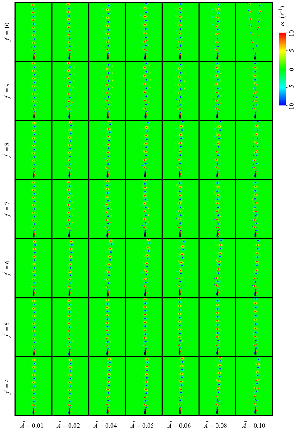
Figure 12. Wake structures generated by the self-propelled pitching foil with perturbations.
