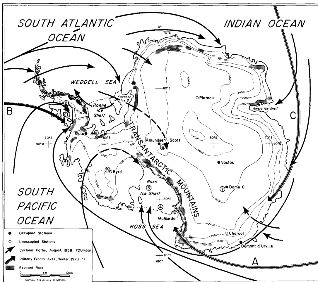
Fig.1. Location of Antarctic surface sampling sites: (1) Monteverti Peninsula, (2) snow-field above Horse Bluff, (3) base camp on RIS, (4) Q-13 on RIS, (5) Byrd station strain network, (6) South Pole station, (7) Dome C. The very heavy lines locate the mean winter position of the major frontal axes (Carleton 1981) which occur in association with the long wave troughs. The lighter arrows trace IGY observations of cyclonic paths during August 1958 (Alt and others 1959).
