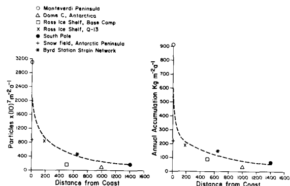
Fig.5. The left diagram represents the relationship between particle concentrations and distance from the coast for seven Antarctic sample sites. On the right is the plot of annual water accumulation vs distance from the coast for each location.
