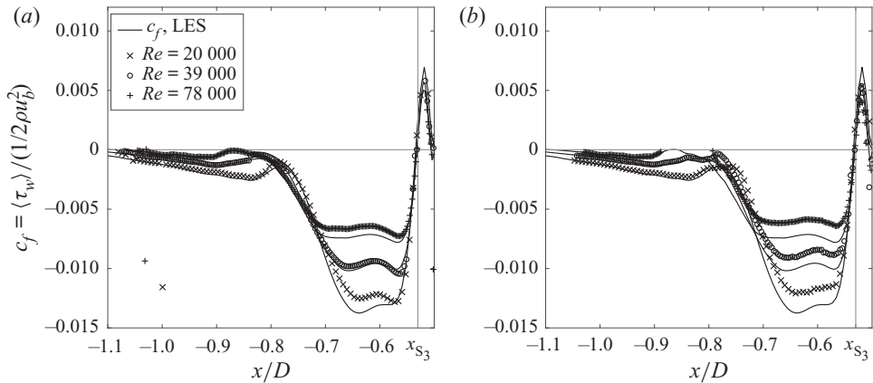
Figure 23. Friction coefficient c_f obtained from the first grid point of the LES data (solid lines), and the Falkner–Skan profiles (symbols) using (a) the best fit and (b) (6.9) to determine the values of \beta .
