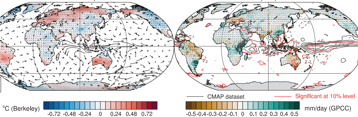
c. SON IOD teleconnection for 2m-temperature/10m-wind
