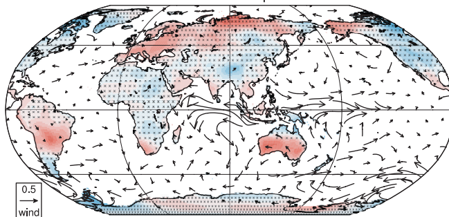
c. SON IOD teleconnection for 2m-temperature/10m-wind
