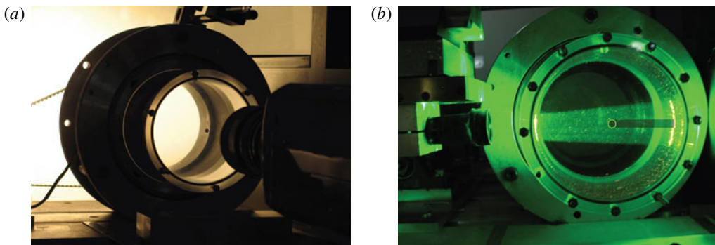
FIGURE 2. Experimental optical set-up. (a) Force measurements. The position, size and shape of the bubble are determined from images recorded with a backlight on a fast camera located in front of the tank. (b) Surrounding flow investigation. The surface spinning and the wake behind the bubble at its equilibrium position are visualized with a laser sheet as shown. With this lighting, a shadow appears behind the bubble on the bubble side that is opposed to the laser source. The fast camera (not visible in the figure) is still positioned in front of the tank.
