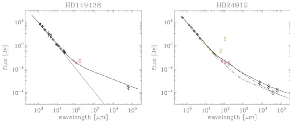
Figure 1. Different computed SED models including microclumping structure of the wind built from IR/radio continuum archival measurements (black and green symbols) and PACS fluxes at 70,100 and 160 \mu\text{m} (red symbols). Arrows denote upper limits. Left: \tau Sco PACS flux values agree with the new unclumped model , f_{\text{cl}}=1 , computed for \dot{M} = 3.23 \times 10^{-7} M_{\odot} \text{yr}^{-1} (black solid line). The blue line represents \tau Sco SED for spectral index \alpha = 2 . Right: \xi Per. Clumping models by Puls et al. (2006); Solid line: \dot{M} = 2.3 \times 10^{-6} M_{\odot} \text{yr}^{-1} and f_{\text{clin}} = 2.1 , f_{\text{clmid}} = 5 , f_{\text{clout}} = 1 ; dotted-dashed line: \dot{M} = 1.2 \times 10^{-6} M_{\odot} \text{yr}^{-1} , f_{\text{clin}} = 8 , f_{\text{clmid}} = 20 , f_{\text{clout}} = 1 ; dashed-triple dotted line: \dot{M} = 1.2 \times 10^{-6} M_{\odot} \text{yr}^{-1} , f_{\text{clin}} = 8 , f_{\text{clmid}} = f_{\text{clout}} = 1 . PACS data break the degeneracy between models pointing to lower mass-loss and clumping structure in the intermediate wind region.
