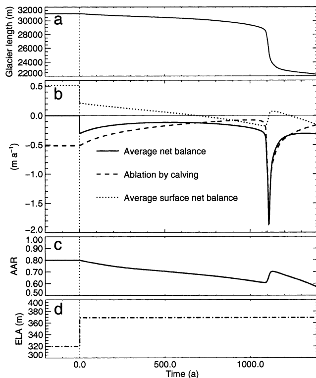
Fig. 7. Mass-balance changes over time for the retreating scenario. At time zero the shift in the mass-balance function was performed and the model calculations were started. (a) Glacier length over time. (b) Net balance, surface net balance (surface accumulation and ablation without calving) and ablation by calving are shown over time as values averaged over the glacier area. (c) AAR over time. (d) ELA as an index for the input mass-balance function over time.
