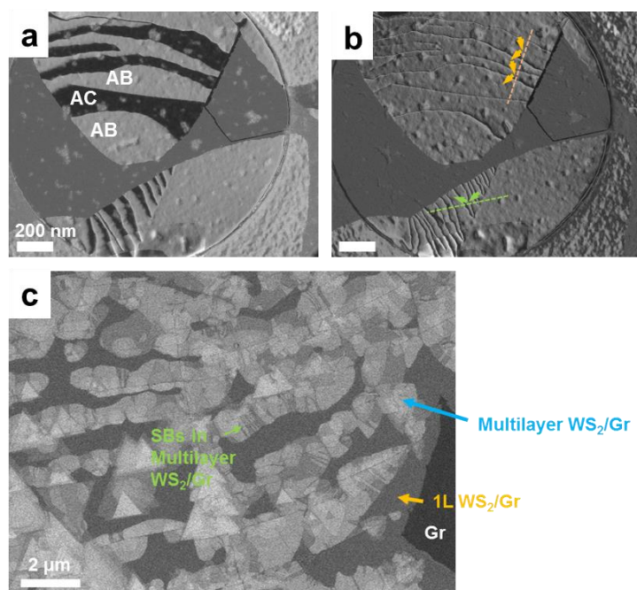
Figure 1. (a-b) Dark-field TEM images obtained by (a) (0\bar{1}10) (1 st ) and (b) (\bar{2}110) (2 nd ) diffraction spots, respectively. (a) and (b) indicate stacking order and layer number, respectively. Orange and green arrows in burgers vector of partial dislocations using adjacent 2 nd order dark-field images. (c) SEM image using backscattered electron mode, showing stacking order. SBs are formed near the graphene wrinkles.
