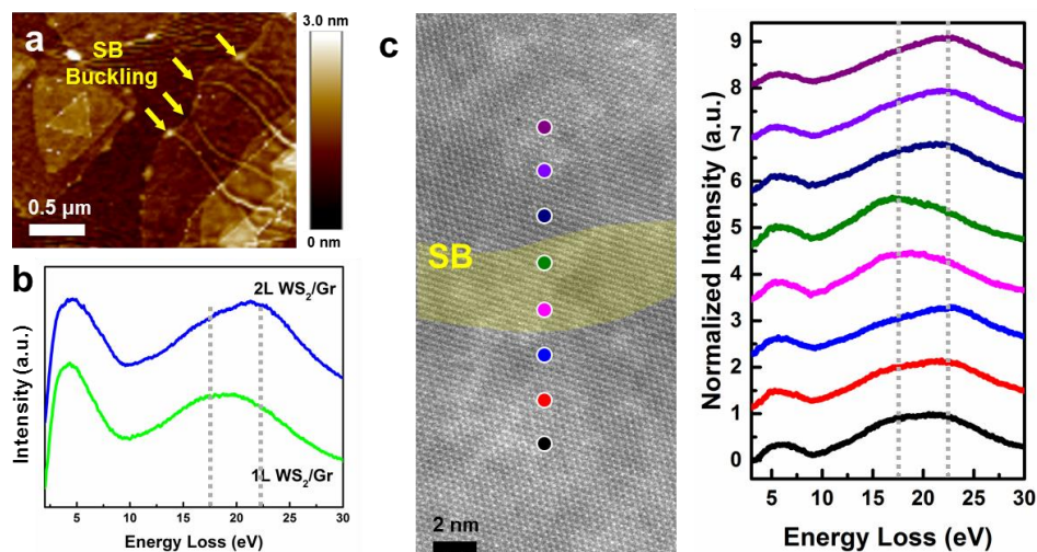
Figure 2. (a) Height image using AFM, showing 1 nm of vertical height at SBs. (b-c) EELS line profile across the SB [5].
