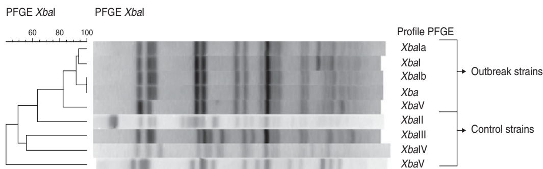
Fig. 2. Dendrogram generated by BioNumerics showing the results of cluster analysis on the basis of PFGE fingerprinting. Similarity analysis was performed using the Dice coefficient, and clustering was by UPGMA. The five PFGE profiles of the strains of the outbreak in Flemish Brabant were compared to different profiles of strains isolated from patients without travel information or having travelled to Egypt. Dendrogram showing the results of cluster analysis on the basis of PFGE fingerprinting of five Shigella sonnei isolates from the outbreak in Flemish Brabant and three controls taken from patients with no travel information or travel to Egypt.
