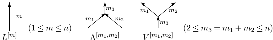
Figure 2: Elementary MOY diagrams
