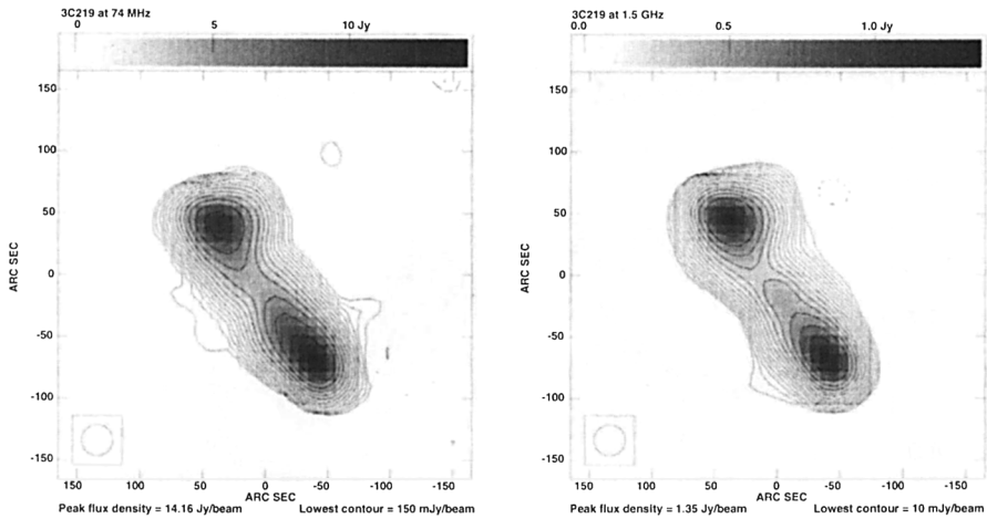
Figure 3. Images of 3C 219 at 74 MHz and 1.5 GHz with 25'' resolution. These images, especially their silhouettes, are more remarkable for their similarities than for their differences.
