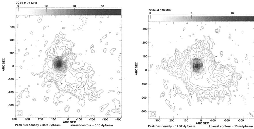
Figure 1. Images of 3C84 at 74 MHz and 330 MHz with 25'' resolution.
