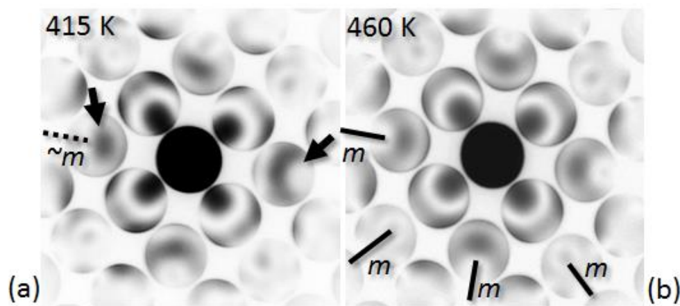
Figure 1. Energy-filtered [100] CBED patterns of the cubic phase of BaTiO 3 taken at specimen temperatures of (a) 415 K and (b) 460 K. The pattern (a) exhibit clear breaking of the fourfold rotation symmetry expected from the cubic phase, while the pattern (b) shows almost the fourfold rotation symmetry.
