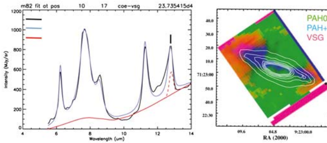
Fig. 4. Example of fit (blue line), using the template spectra of Figure 2 (corrected for extinction on the line of sight), to an observed mid-IR spectrum taken in the cube of M82 in the outflow region. Achieving the fit on all the spatial positions of the spectral cube, the spatial distribution map of the PAH/eVSG populations can be built (inset). In the inset, white contours show the 3.6\ \mu\text{m} -mostly- stellar emission.
