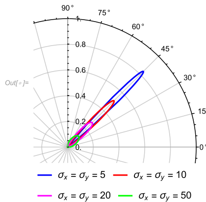
Figure 30. Polar plot showing the probability of geometric intrusion for perpendicular velocities for full normal distribution with \rho = 1 ( \mu = 90 and \nu = 90 , l = 15 , u = 180 ) for a range of equal standard deviations. The radius coordinate represents conflict probability magnitude, while the angle coordinate shows relative azimuth.
