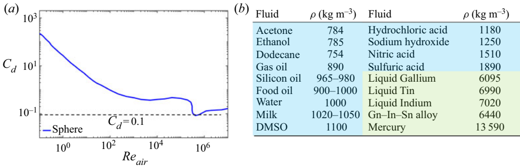
Figure 13. (a) Drag coefficient, C_d , for a sphere as a function of Reynolds number Re_{air} = ud/v_a , where v_a is the air kinematic viscosity. (b) Density values for common liquids at room temperature.
