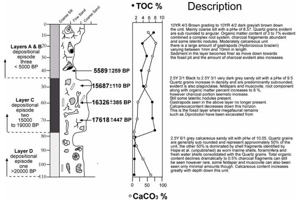
Figure 2 Stratigraphical reconstruction of the Black Creek Swamp fossil excavation pit. Included are PH w values, 14 C dates, and TOC data provided with δ 13 C values from the Rafter Isotope Lab, Lower Hutt, New Zealand.
