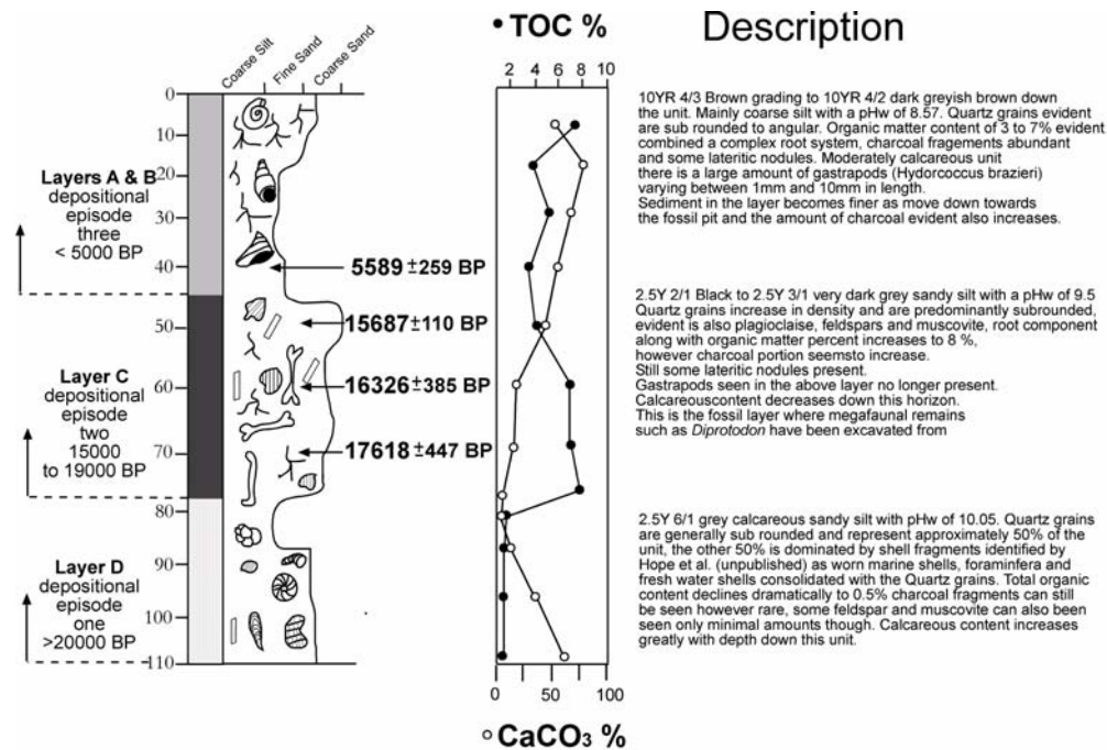
Figure 2 Stratigraphical reconstruction of the Black Creek Swamp fossil excavation pit. Included are \text{pH}_w values, ^{14}\text{C} dates, and TOC data provided with \delta^{13}\text{C} values from the Rafter Isotope Lab, Lower Hutt, New Zealand.
