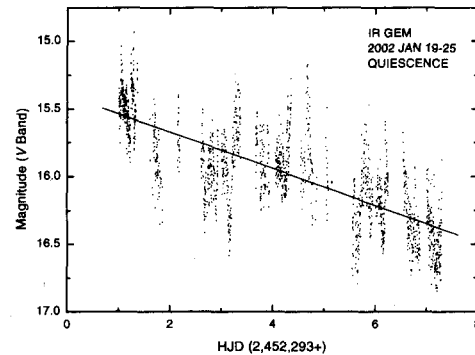
Fig. 1. Full light curve of the observations. The ordinate presents the estimated magnitudes based on a comparison star V magnitude of 13.761(30). The solid line shows the best linear fit to the data.
