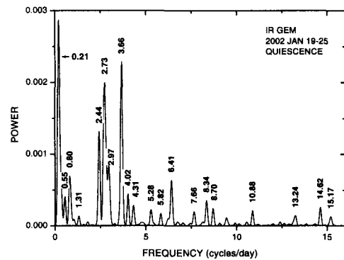
Fig. 3. CLEAN spectrum of the complete set of the de-trended time series, showing a strong signal at 0.21 c/d. The complicated pattern suggests multi-periods. Spikes at 14.62 and 15.17 c/d can also be seen.
