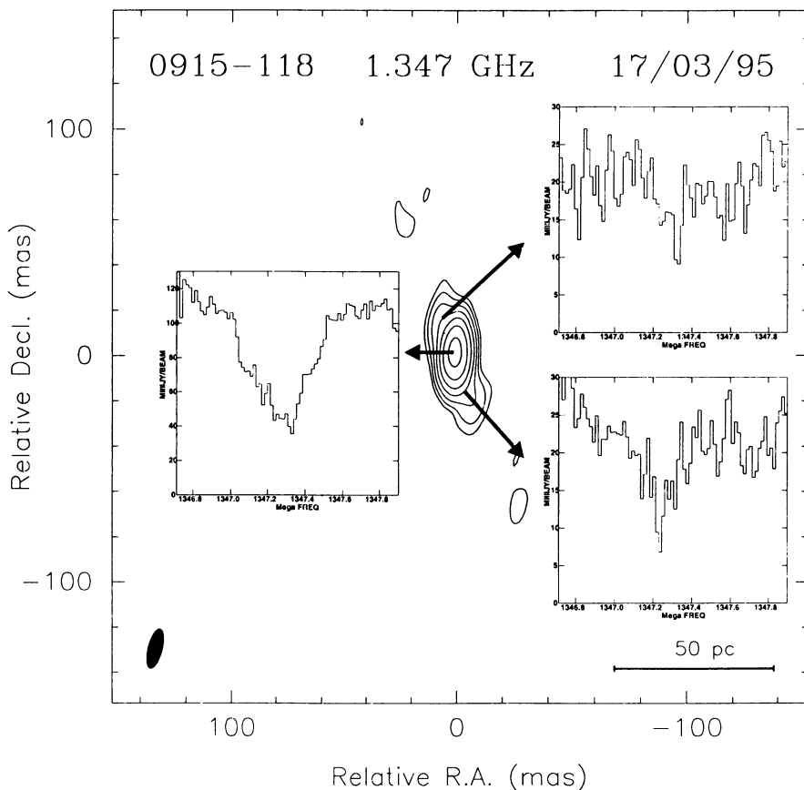
Figure 2. HI absorption against the nucleus of Hydra A. Contours are at -1, 1, 2, 4, 8, 16, 32, and 64 mJy/beam with a beam size of 18 \times 6 mas in p.a. -14^\circ . The total velocity spanned by the inset figures is 250 \text{ km s}^{-1} with a spectral resolution of 3.5 \text{ km s}^{-1} .
