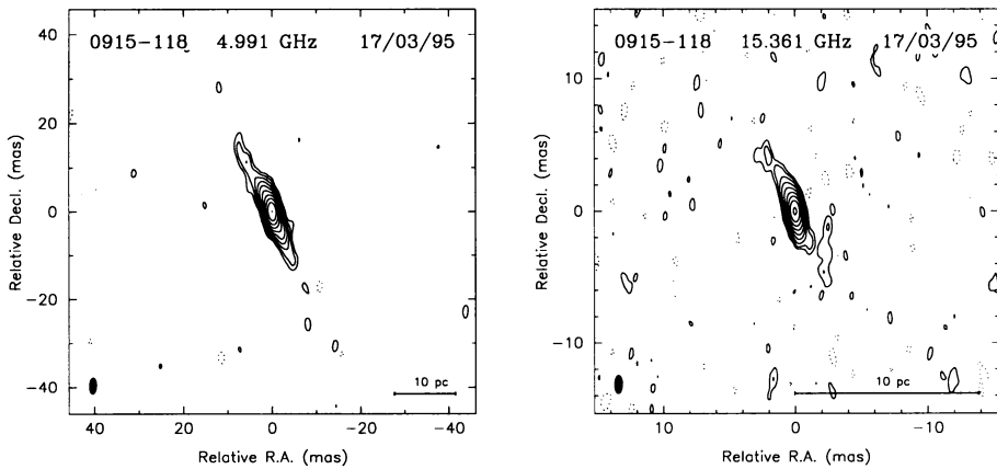
Figure 1. a. The nucleus of Hydra A at 5 GHz. Contours are drawn at -0.3, 0.3, 0.6, 1.2, 2.4, 4.8, 9.6, 19.2, 38, 77, and 154 mJy/beam where the beamsize is 3.66 \times 1.53 mas in p.a. -3^\circ . b. The nucleus of Hydra A at 15 GHz. Contours are at -0.5, 0.5, 1, 2, 4, 8, 16, 32, 64, and 128 mJy/beam where the beamsize is 1.38 \times 0.58 mas in p.a. -1^\circ .
