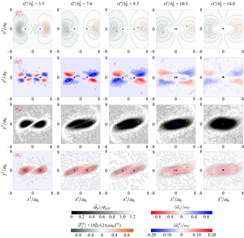
Figure 10. Iso-contours of ensemble-averaged and filtered antisymmetric particle-feedback force along the two vortex centres \langle \bar{F}_\parallel^A \rangle , antisymmetric axial vorticity \langle \bar{\omega}_z^A \rangle , particle volume fraction \langle \phi_p \rangle and total axial vorticity \langle \bar{\omega}_z \rangle at representative times during the merger. Data correspond to case F with St_\Gamma = 0.2 , M = 1 and Re_\Gamma = 530 .
