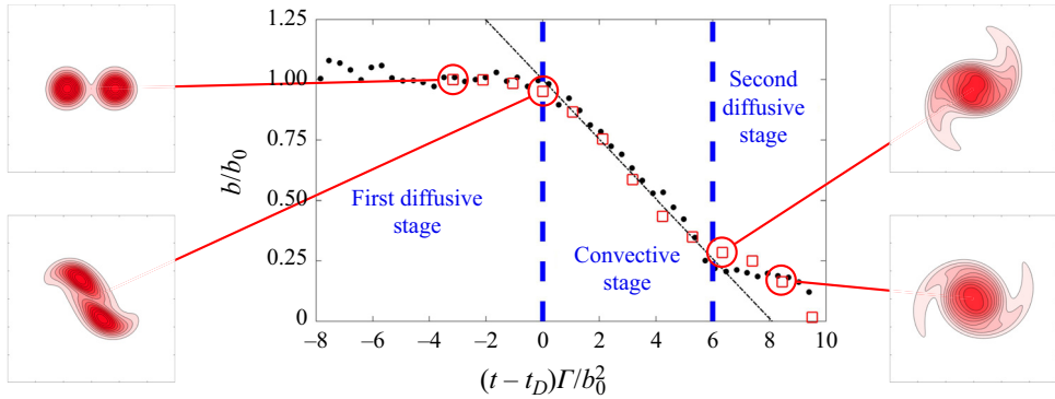
Figure 1. The evolution of vortex separation b/b_0 as a function of time in a single-phase fluid at Re_\Gamma = 530 . Symbols: ●, Cerretelli & Williamson (2003); □, present simulation. Snapshots represent normalized vorticity.
