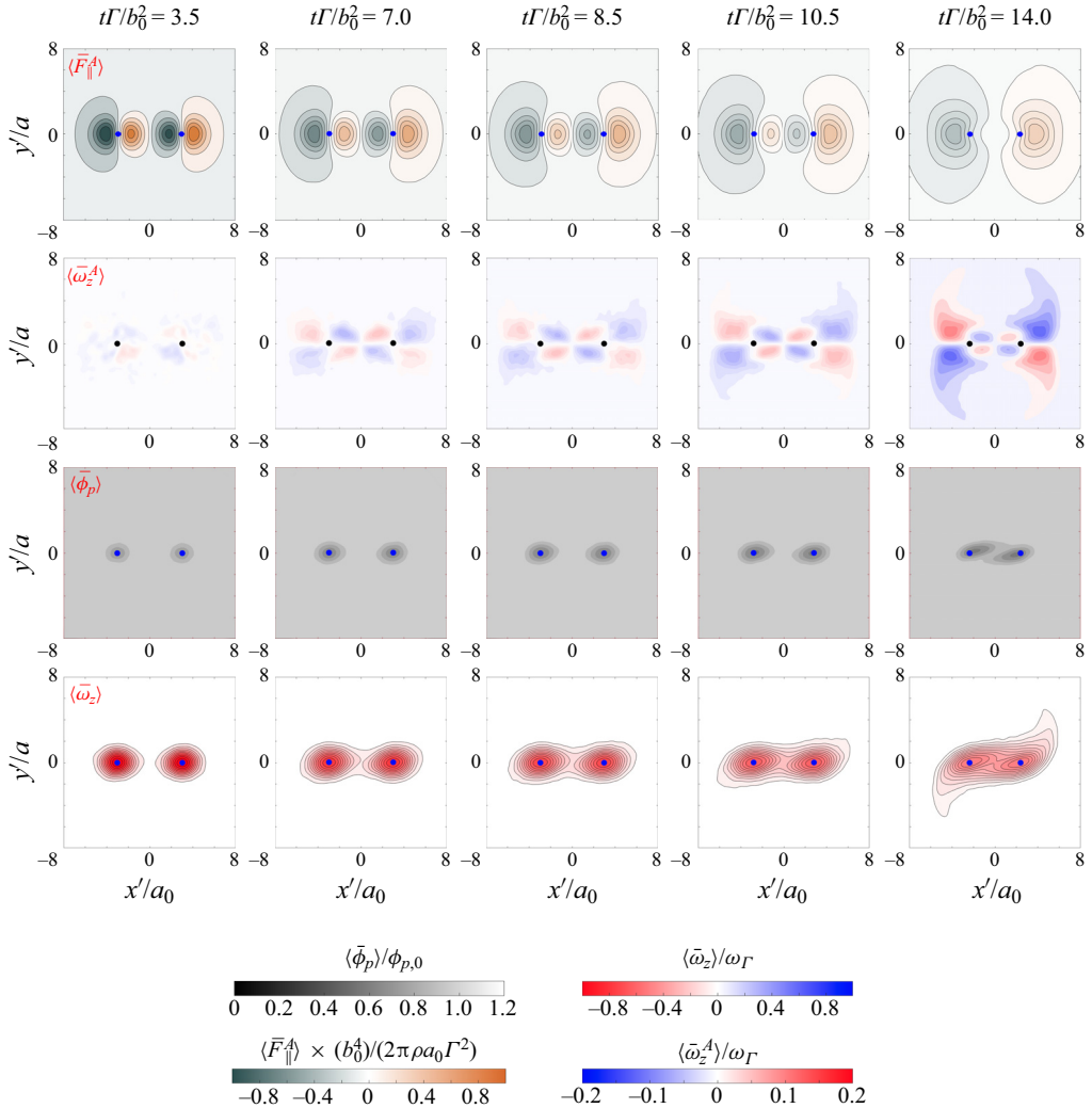
Figure 8. Iso-contours of ensemble-averaged and filtered antisymmetric particle-feedback force along the two vortex centres ( \bar{F}_{\parallel}^A ), antisymmetric axial vorticity ( \bar{\omega}_z^A ), particle volume fraction ( \bar{\phi}_p ) and total axial vorticity ( \bar{\omega}_z ) at representative times during the merger. Data correspond to case B with St_{\Gamma} = 0.01 , M = 1 and Re_{\Gamma} = 530 .
