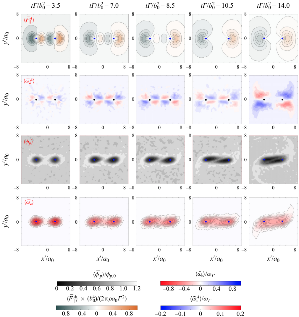
Figure 9. Iso-contours of ensemble-averaged and filtered antisymmetric particle-feedback force along the two vortex centres \langle \bar{F}_{\parallel}^A \rangle , antisymmetric axial vorticity \langle \bar{\omega}_z^A \rangle , particle volume fraction \langle \bar{\phi}_p \rangle and total axial vorticity \langle \bar{\omega}_z \rangle at representative times during the merger. Data correspond to case D with St_{\Gamma} = 0.05 , M = 1 and Re_{\Gamma} = 530 .
