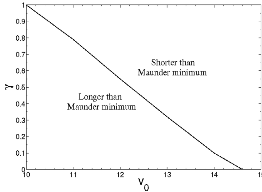
Figure 2. Parameter space of amplitude of MC ( v_0 ) and polar field reduction factor ( \gamma ). The line shows the values of these parameters which are giving Maunder-like grand minima.
