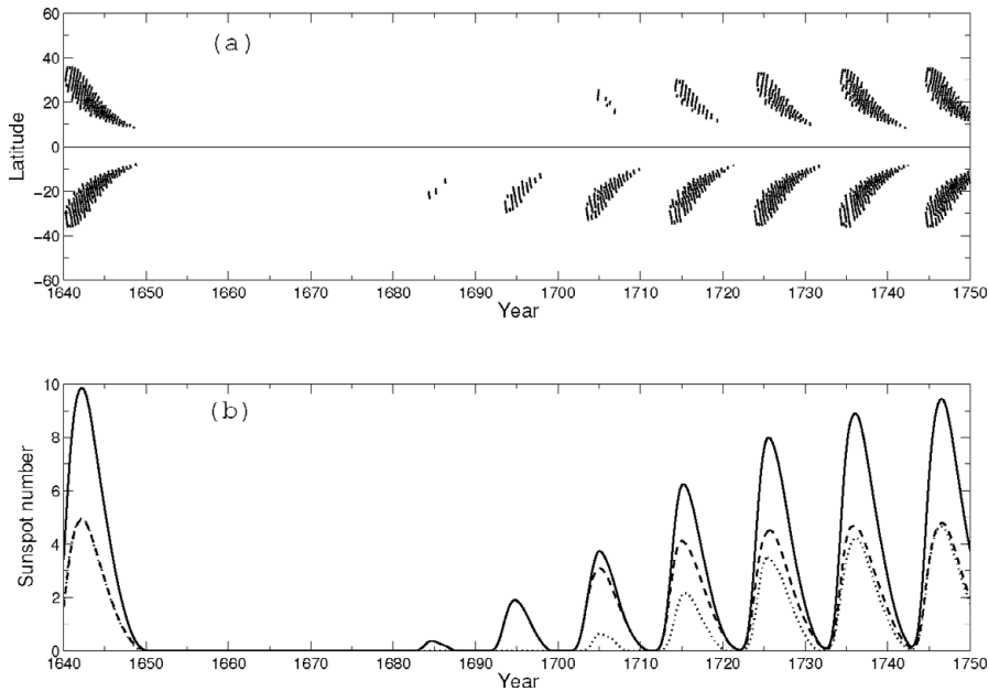
Figure 1. Results covering the Maunder minimum episode. (a) The butterfly diagram. (b) The smoothed sunspot number. The dashed and dotted lines show the sunspot numbers in southern and northern hemispheres, whereas the solid line is the total sunspot number. From Choudhuri & Karak (2009).
