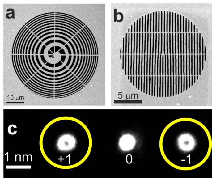
Fig 1: Generation of electron vortex beams. a, Scanning electron microscope image of a spiral-type aperture. b, Scanning electron microscope image of a fork-type aperture. c, Image of the electron beam that is generated by the fork-type aperture in b. Yellow circles mark the area of the inserted additional aperture that is used for the generation of single EVB.
