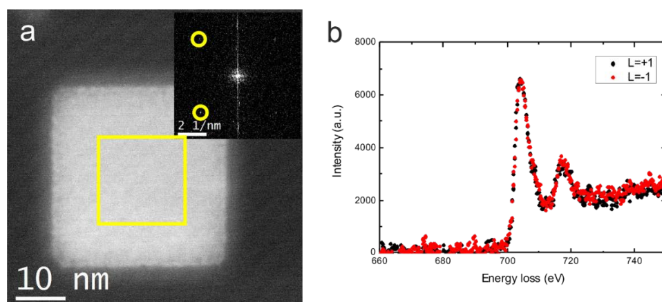
Fig 2. Magnetic measurements using a spiral-type aperture at FePt nanocubes. a, Scanning dark-field image of a FePt nanocube acquired with the L=0 beam of the spiral-type aperture. Inset show FFT with marked superstructure reflections of L1_0 -ordered FePt. b, EEL spectra acquired with an EVB scanned over the yellow marked area in a. No significant EMCD signal (= difference between the two spectra) is observed.
