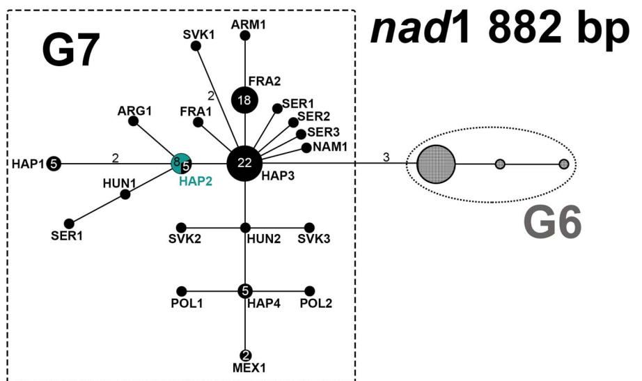
Figure 3. Median-joining network of Echinococcus granulosus s.l. G7 isolates from Cape Verde and respective G6–G7 reference sequences from GenBank based on NADH dehydrogenase subunit 1 ( nad1 , 882 bp) gene fragment. Cape Verde sequences of the current study obtained from tissue ( n=7 ) and fecal samples ( n=1 ) are depicted in green. References from GenBank of genotype G6 are represented schematically, and references of G7 are depicted in black. Numbers inside the circles represent the number of identical sequences within the respective haplotype; numbers beside the lines represent the number of mutations. Haplotype names are designated as 3 letter abbreviations [HAP, haplotypes representing samples originating from different countries; ARG, Argentina; ARM, Armenia; FRA, France (Corsica); HUN, Hungary; MEX, Mexico; NAM, Namibia; POL, Poland; SER, Serbia; SVK, Slovakia].
