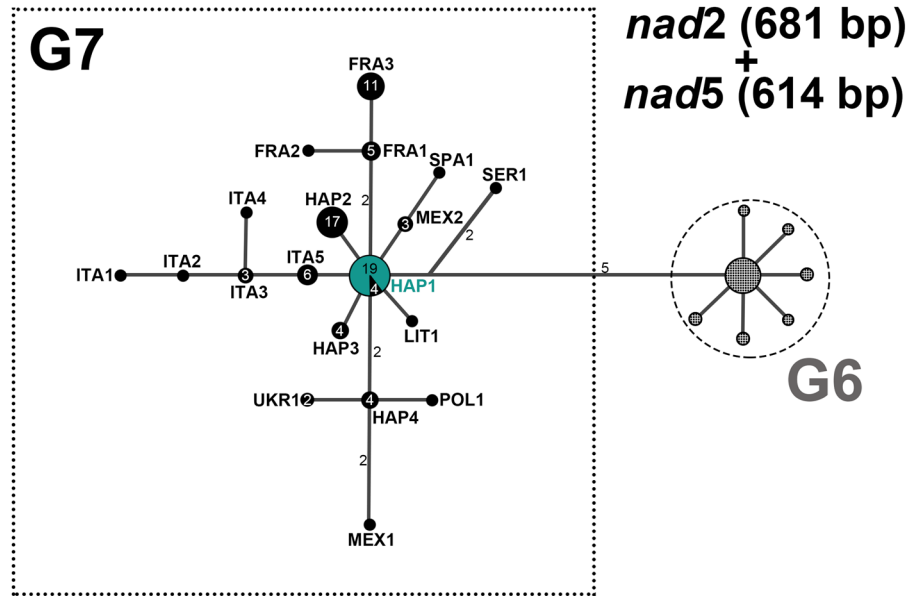
Figure 2. Median-joining network of Echinococcus granulosus s.l. G7 isolates from Cape Verde and respective G6–G7 reference sequences from GenBank based on gene fragments of concatenated NADH dehydrogenase subunits 2 ( nad2 , 681 bp) and 5 ( nad5 , 614 bp). Cape Verde sequences of the current study obtained from tissue ( n=13 ) and fecal samples ( n=7 ) are depicted in green. References from GenBank of genotype G6 are represented schematically, and references of G7 are depicted in black. Numbers inside the circles represent the number of identical sequences within the respective haplotype; numbers beside the lines represent the number of mutations. Haplotype names are designated as 3 letter abbreviations [HAP, haplotypes representing samples originating from different countries; FRA, France (Corsica); ITA, Italy; LIT, Lithuania; MEX, Mexico; POL, Poland; SER, Serbia; SPA, Spain; UKR, Ukraine].
