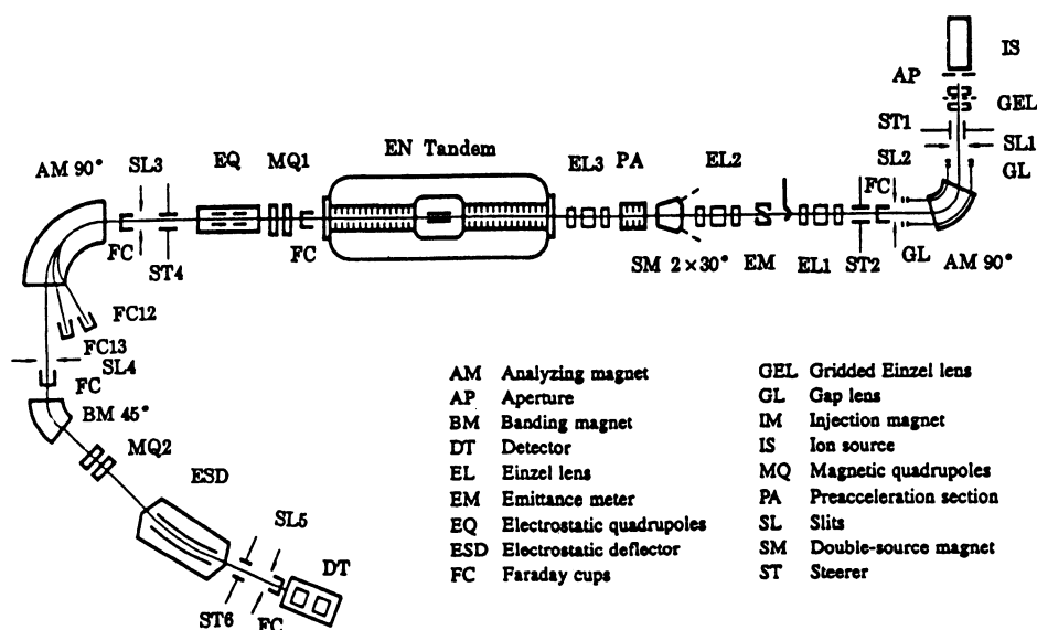
Fig. 1. Schematic layout of PKUAMS
