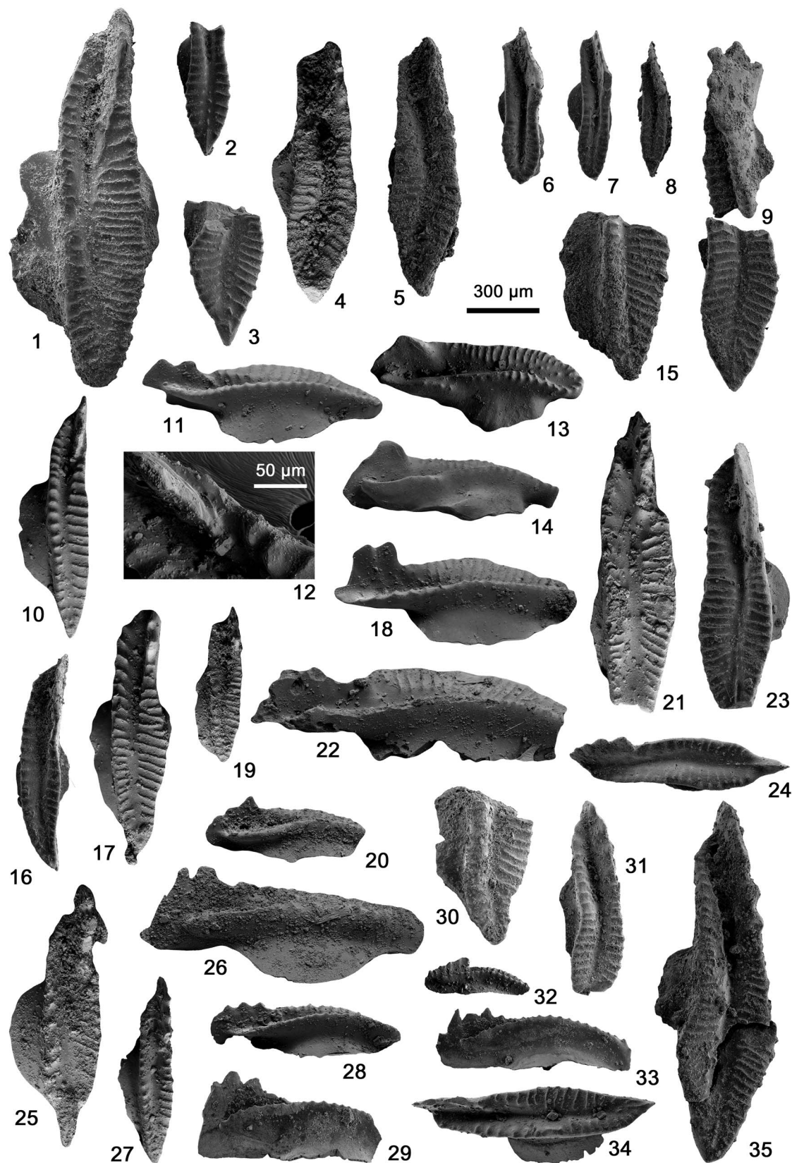
Figure 4. Conodonts from Yashui-A section (1, 10–22, 25, 27–30, 33, 34 are sinistral Pa elements; 2–9, 23, 24, 26, 31, 32, 35 are dextral Pa elements). (1–26) Cavusgnathus aff. Cav. unicornis Youngquist and Miller, 1949: (1, 2, 7, 8, 10–14) 201189, 201190, 201195, 201196, 201198, 201198, 201198, 201199, 201199, bed 63; (3) 201191, bed 1; (4, 26) 201192, 201192, bed 55; (5, 6) 201193, 201194, bed 57; (9, 15) 201197, 201200, bed 67; (16–18) 201201, 201202, 201202, bed 69; (19, 20) 201203, 201203, bed 91; (21–24) 201204, 201204, 201205, 201206, bed 99; (25) 201207, bed 53. (27–35) Cavusgnathus unicornis Youngquist and Miller, 1949: (27, 28) 201208, 201208, bed 100b; (29, 33–35) 201209, 201213–201215, bed 104; (30–32) 201210–201212, bed 103. (1–11, 13–35) Scale bars = 300 µm; (12) scale bar = 50 µm.
