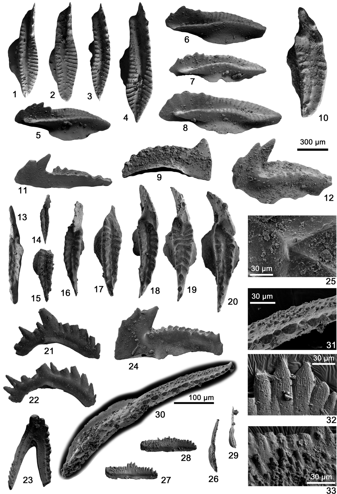
Figure 5. Conodonts from Yashui-A section (1, 2, 5, 6, 14–17, 26, 29–31 are sinistral Pa elements; 3, 4, 7–13, 18–20, 24, 25, 27, 28, 32, 33 are dextral Pa elements; 21, 22 are Pb elements; 23 is S element). (1–8) Cavusgnathus unicornis Youngquist and Miller, 1949: (1, 2, 4–6, 8) 201216, 201217, 201219, 201216, 201217, 201219, bed 105; (3, 7) 201218, 201218, bed 104. (9) Hindeodus cristulus (Youngquist and Miller, 1949), 201220, bed 57. (10–20, 24, 25) Clydagnathus windsorensis (Globensky, 1967): (10, 12) 201221, 201221, bed 57; (11, 13, 14) 201222, 201222, 201223, bed 51; (15–18, 24) 201224–201227, 201227, bed 63; (19, 20, 25) 201228, 201229, 201228, bed 69. (21) Ozarkodina sp., 201230, bed 69. (22) Ozarkodina sp., 201231, bed 63. (23) Apatognathus sp., 201232, bed 105. (26–33) Vogelgnathus campbelli (Rexroad, 1957): (26–28, 30–33) 201233–201235, 201233, 201233–201235, bed 104; (29) 201236, bed 103. (1–24, 26–29) Scale bars = 300 μm; (25, 31–33) scale bars = 30 μm; (30) scale bar = 100 μm.
