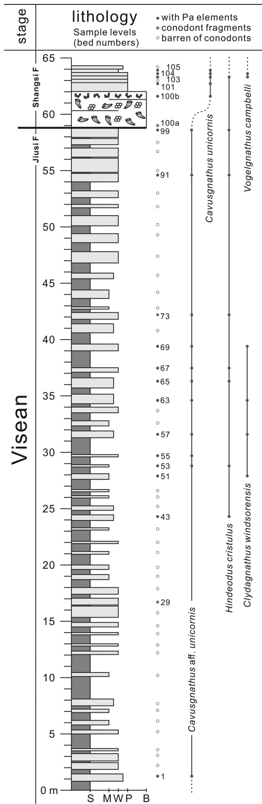
Figure 3. Lithostratigraphic column and conodont distributions of the Yashui-A section. F = formation; S = shaly marls; M = mud limestone; W = wackestone; P = packstone; B = biostrome.
