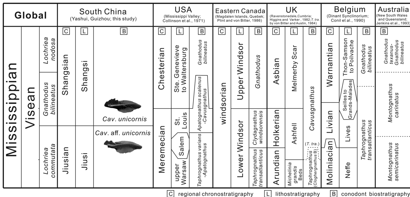
Figure 7. Correlation of the biozonations based on the shallow-water conodonts during the Visean of different regions.
