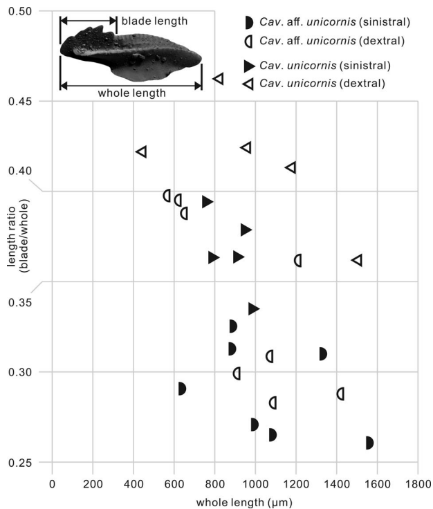
Figure 6. Plot of the dimensional ratios of Cavusgnathus unicornis and Cavusgnathus aff. Cav. unicornis
