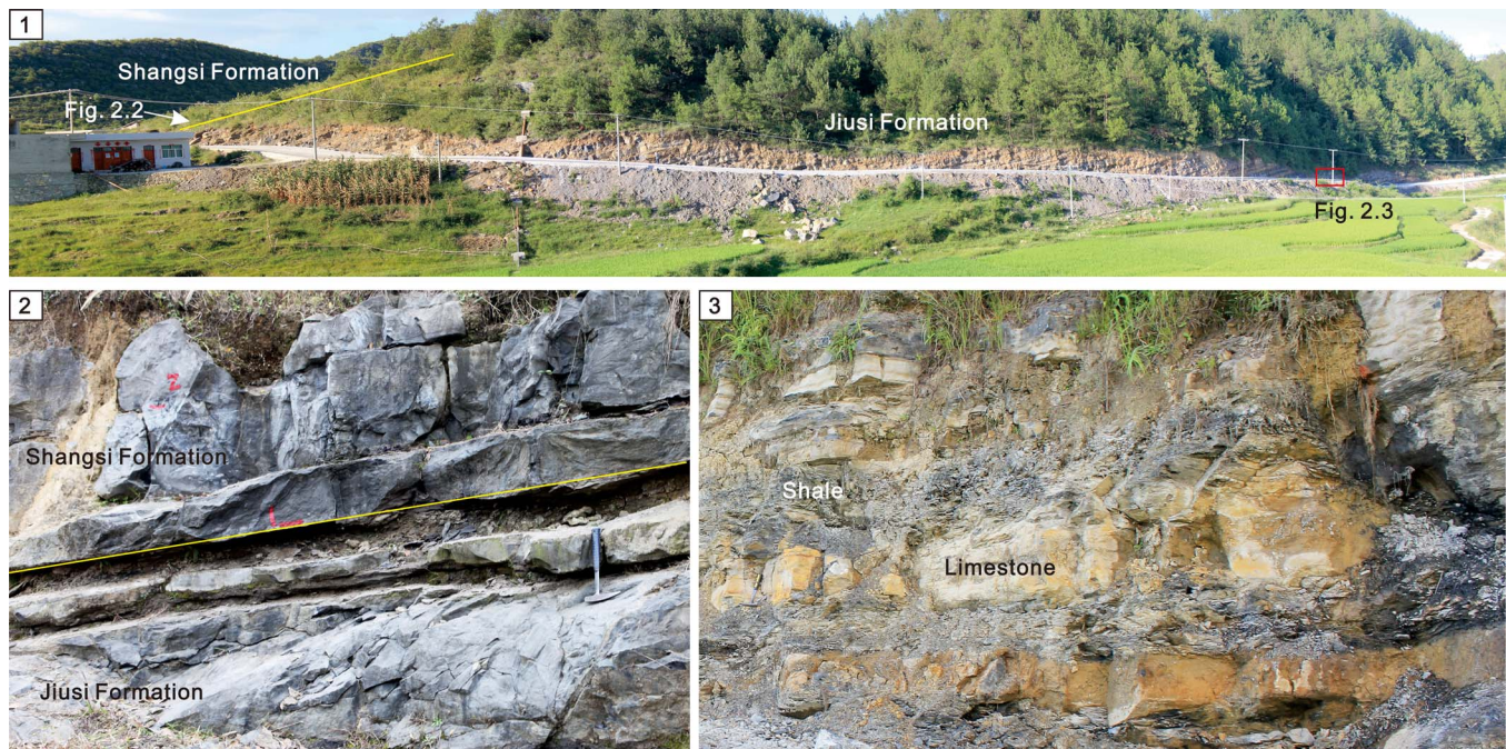
Figure 2. Outcrop pictures of the Yashui-A section. (1) Distant view of the section. (2) Detail of the section showing the boundary between the Jiusi Formation and the Shangsi Formation. (3) Typical lithostratigraphic succession of the Jiusi Formation.
