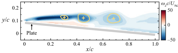
Figure 9. Spanwise vorticity field in the plane z/c = 0 at \theta = 0^\circ . The LEV heads are presented by the contour lines of Q_{2-C} c^2/U_\infty^2 = 30 in yellow, with the central positions marked by the yellow crosses.
