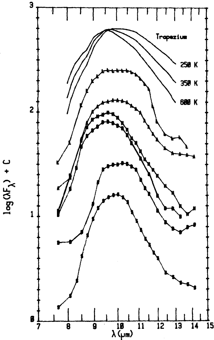
Fig. 8. Observed relative emission spectra for small ( 0-2\mu ) grains at \sim 600 K from the laboratory measurements of Rose (1977) for Lunar soil 15531 (L), a melted anorthite (A), Montmorillonite (M), Columbia River Basalt (B), Dunite (D), and amorphous silicate (S). The observed emission from the Orion Trapezium is shown (Forrest et al., 1975) renormalized from assumed 250 K grains to 350 K and 600 K grains for comparison.
