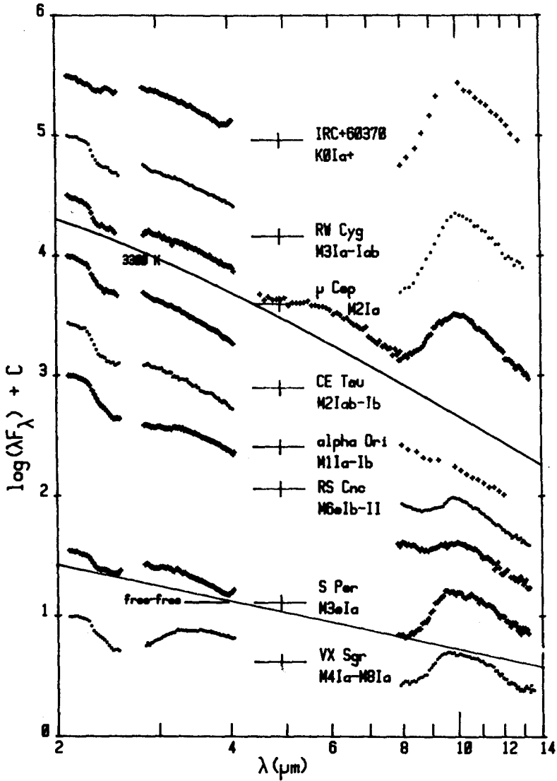
Fig. 5. Relative \lambda\lambda 2-13 \mu spectrophotometry of representative luminous cool stars (M and K supergiants). A 3300 K blackbody and a free-free slope are included for comparison.
