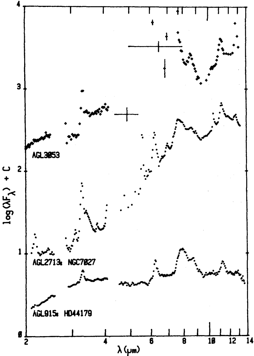
Fig. 12. Relative \lambda\lambda 2-13 \mu spectrophotometry of representative infrared sources with unidentified infrared sources with unidentified emission features at 3.3 \mu /3.4 \mu , 6.2 \mu , 7.9 \mu , 8.6 \mu , and 11.2 \mu . Points with broad horizontal bars are broad bandpass observations.
