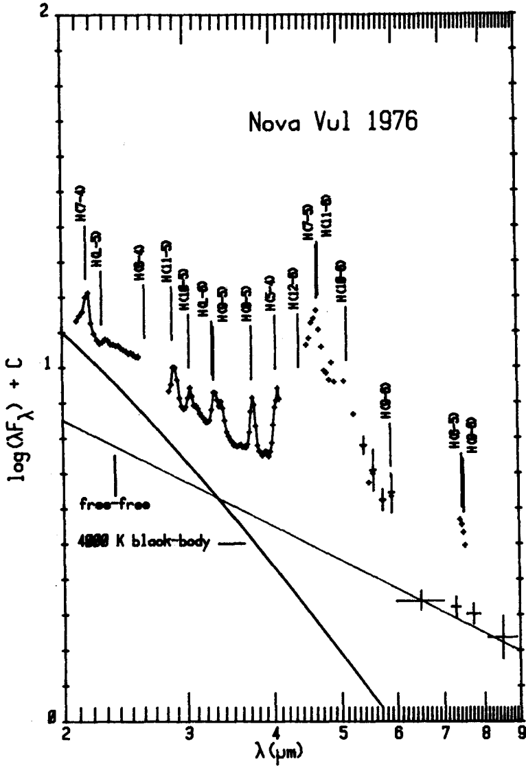
Fig. 10. Spectrophotometry of Nova (NQ) Vulpecula 1976 during the free-free emission phase, taken 31 Oct. 1976 (2-4 \mu ) and 5 Nov. 1976 (4-8 \mu ). Overlapping broad bandpass data agree to +15%. Positions of hydrogen lines are indicated. Energy flux at 3.0 \mu is 3.0 10 -15 w/cm 2 .
