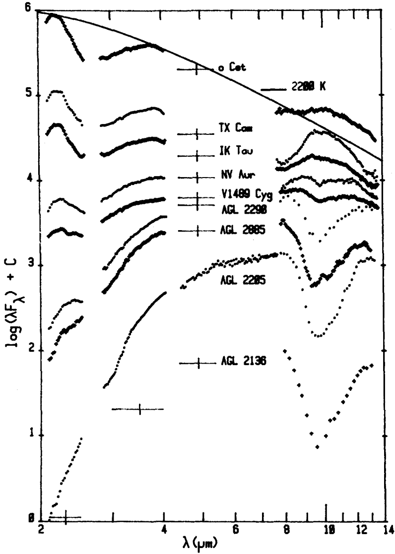
Fig. 6. Relative \lambda\lambda 2-13 \mu spectrophotometry of M stars illustrating the observed range in total optical depth in dusty circumstellar envelopes.
