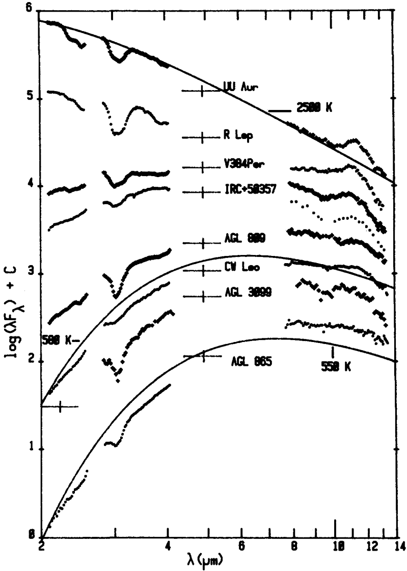
Fig. 9. Relative \lambda\lambda 2-13 \mu spectrophotometry of C stars illustrating the observed range in total optical depth in circumstellar dusty envelopes.
