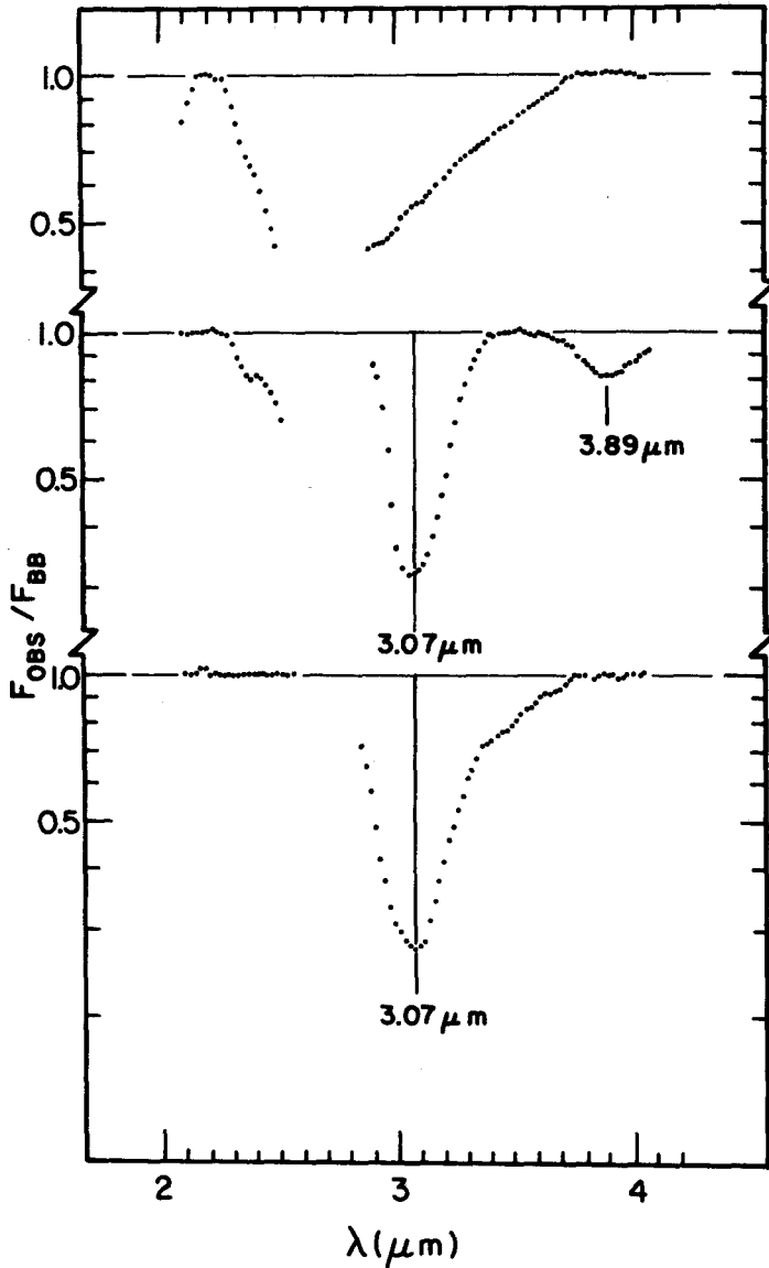
Fig. 2. Observed \lambda\lambda 2-4 \mu absorptance in circumstellar envelopes. Spectra (top to bottom) have been divided by appropriate blackbodies to better define band structure: o Cet (2200 K) an M star; SS Vir (200 K) a C star; and AGL 989 (800 K) a compact infrared source in a molecular cloud with the "interstellar ice" band.
