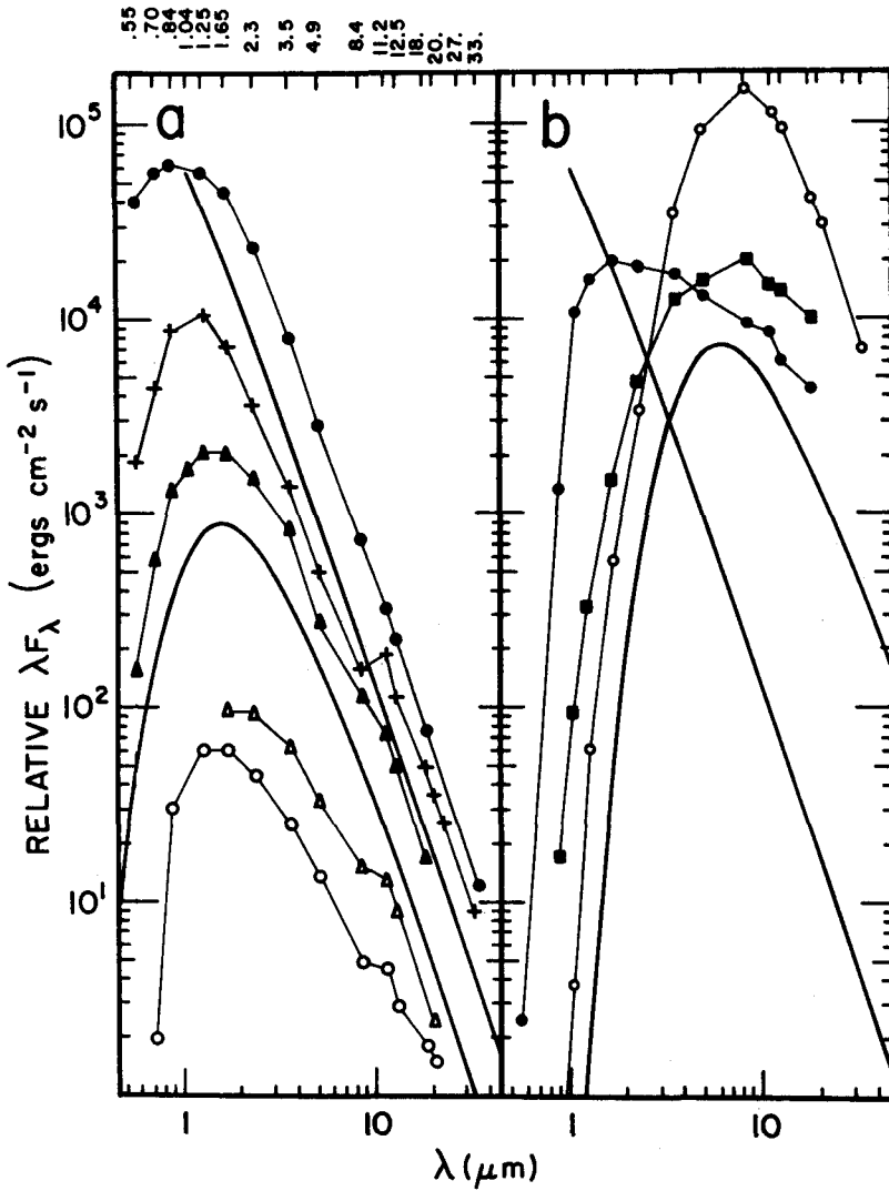
Fig. 3. Relative energy flux of late-type stars with minimal infrared excess consistent with photospheric emission (Panel a) and with large infrared excess indicative of thermalized emission from an extensive dusty circumstellar envelope (Panel b). Stars shown (top to bottom) in Panel a: \alpha Boo (K2 III), \alpha Ori (M2 Ia), UU Aur (C5,4), R Lep (C7,6e), \alpha Cet (gM7e), 10,000 K and 2,400 K blackbodies; Panel b: CW Leo (open circles), IK Tau (filled circles) and V1489 Cyg (squares), 10,000 K and 600 K blackbodies.
