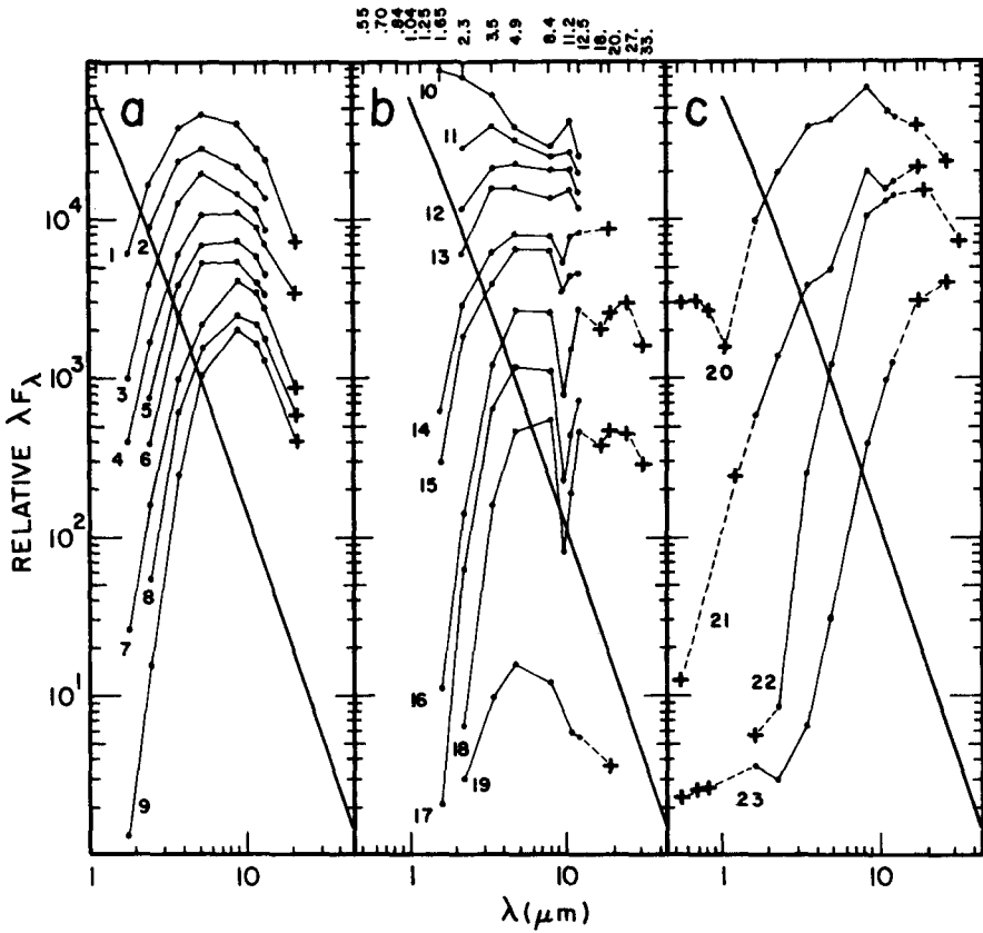
Fig. 4. Relative energy flux of representative objects in the AGL Infrared Sky Survey from MSIII (individual objects are identified in Table I of MSIII). In Panel a are primarily C stars; in Panel b, primarily M stars (or objects with O/C normal); and in Panel c, objects of uncertain evolutionary state surrounded by dense circumstellar disk-like envelopes.
