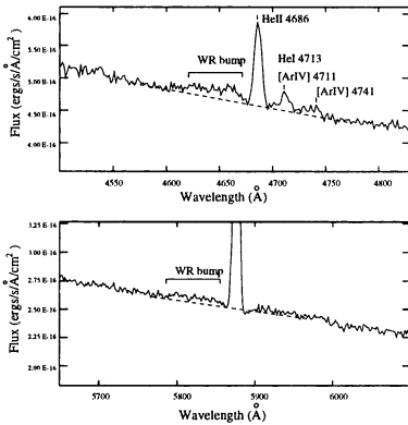
Figure 1. Left: Regions of the spectrum of IZw 18 around the He II 4686 Å (upper) and the He I 5876 Å (lower). The spectrum is integrated over 7''.8 centered on the maximum continuum emission. The broken line shows the position of the fitted continuum.
