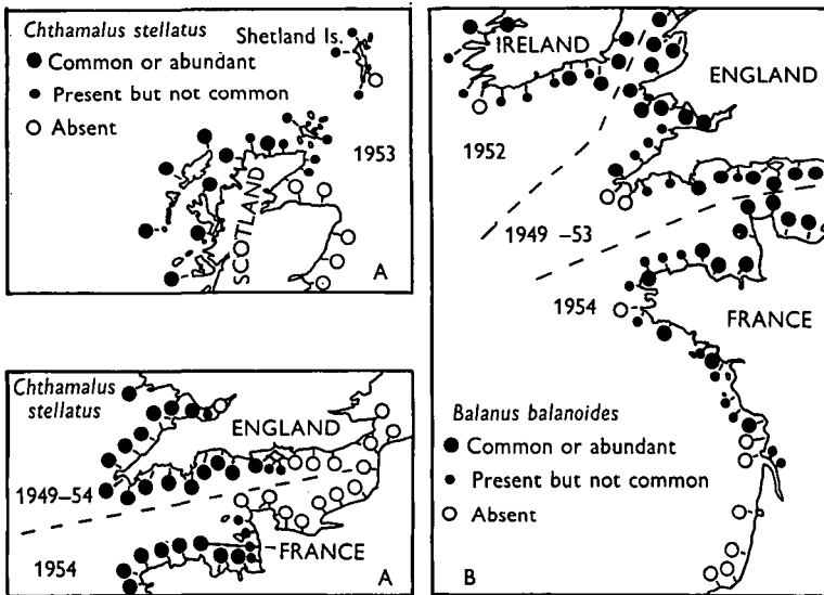
Fig. 1 A. The northern and eastern boundaries of C. stellatus in Europe. B: the known southern and western limits of Balanus balanoides in Europe. In each species, the dividing line between the present and common categories corresponds to a density of approximately 0.5 individuals per square centimetre.
