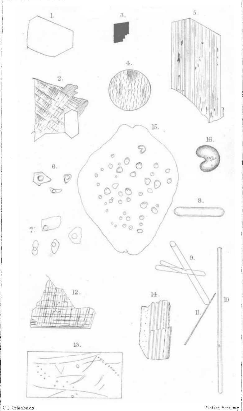
Microscopic Structure of Irish Granites. Figs. 1-6. Granite of Aillemore. Figs. 7-16. Granite of Ballyknockan.
