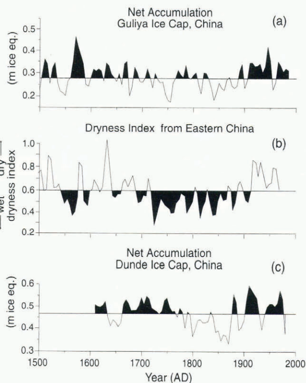
Fig. 7. Net accumulation since 1500 AD on (a) Guliya and (c) Dunde, with (b) the historical dryness index from eastern China from Zhang (1981). Drier conditions on Guliya tend to be associated with wetter conditions in eastern China. The ice-core annual accumulation data were treated identically to Zhang's dust indices; that is, 10 year running means were calculated and every fifth point was plotted. The dryness index ( I_D ) = 2D/N where D is the number of stations with a wetness/dryness grade of 4 or 5 and N is the total number of stations considered. The "yearly charts" were used to compile the data set of 100 stations in eastern China (see Wang and Zhang, 1992, p. 303).
