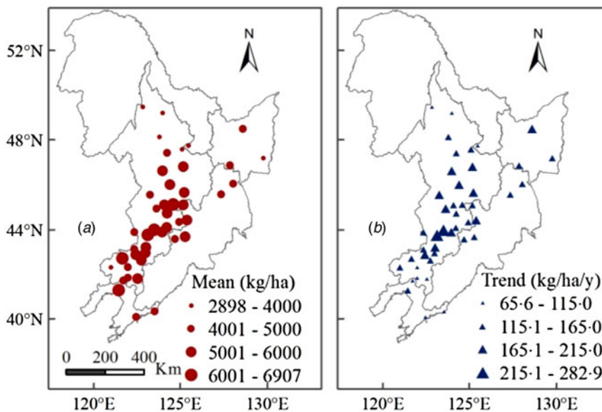
Fig. 10. Distributions of (a) the average maize yield and (b) the maize yield trend from 1961 to 2010 across NFR, the trends for all stations are significant at level P < 0.001 . Colour online.
