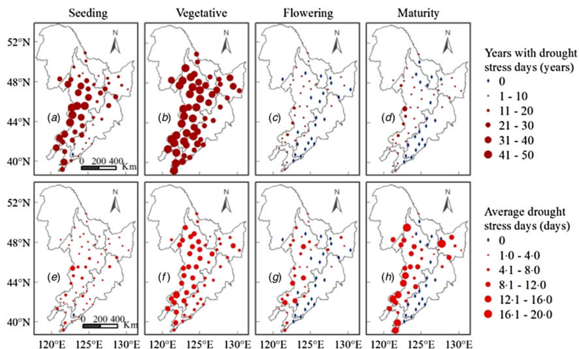
Fig. 7. Spatial variation of (a–d) years with drought stress days and (e–h) average drought stress days excluding the zero values during 1961–2010 in NCR for different maize growth phases, where drought stress days means the days with water deficit, and years with drought stress days represent the number of years that the drought stress days were larger than 0. Colour online.
