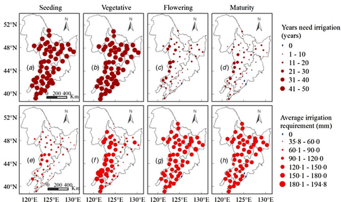
Fig. 9. Spatial variation of (a–d) years which need irrigation and (e–h) average irrigation requirement excluding zero values during 1961–2010 in NFR for different maize growth phases, where the years with need of irrigation represent the number of years that the irrigation requirement was larger than 0. Colour online.
