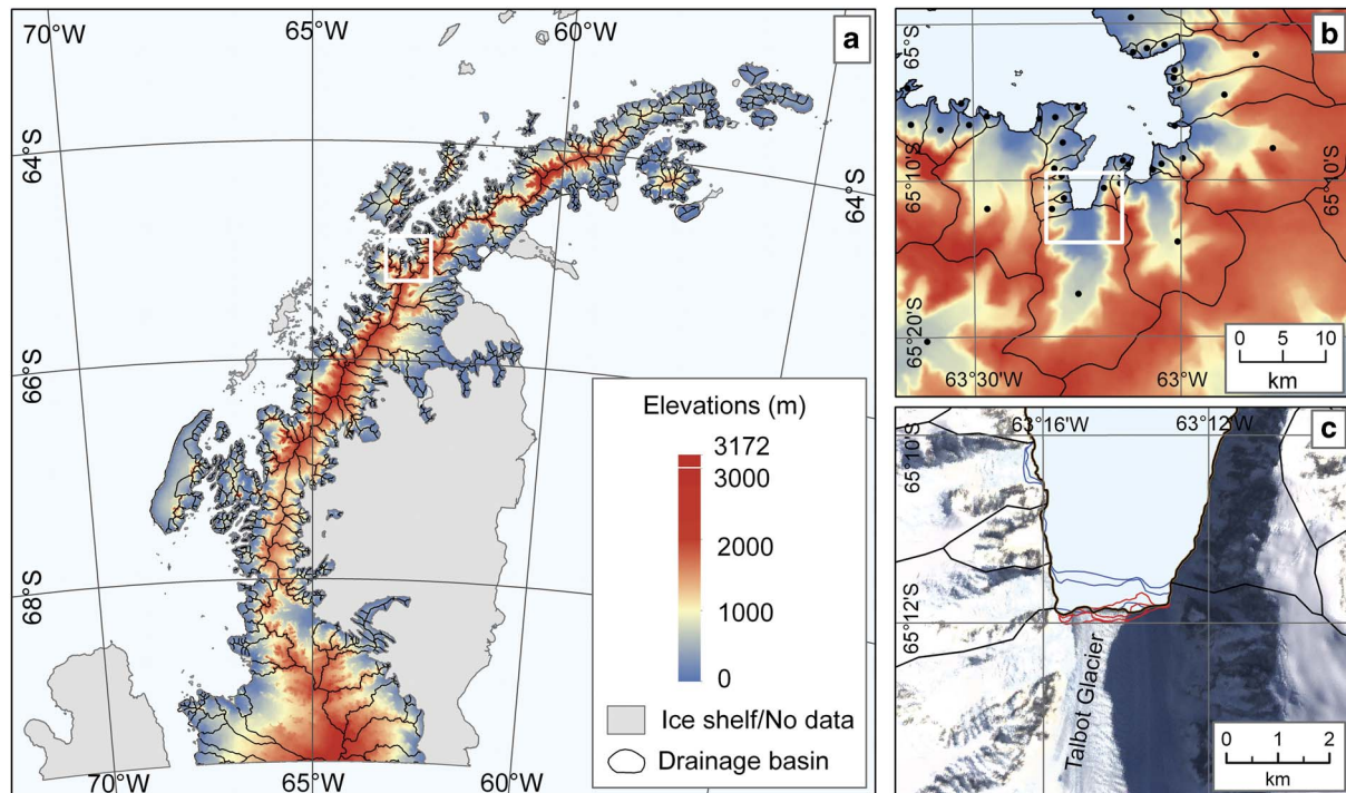
Fig. 1. Glacier drainage basin outlines. a. Shows the spatial extent of the glacier outlines. The white box is the inset shown on b. which illustrates the level of detail of the dataset. The white box on b. indicates the larger scale plot shown in c. which is a sample glacier showing the ice-front data; red lines are post-2000 ice fronts and blue lines are pre-2000. The background image is Landsat ETM+ image LE7218106000105250, 21/02/2001.
