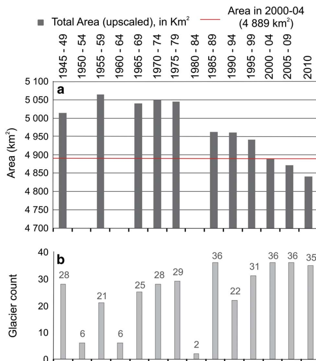
Fig. 9. a. Up-scaled areas for all glaciers with frontal records in nine or more time intervals (36 glaciers). b. Number of glaciers with ice-front positions in each interval.
