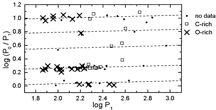
Figure 3. C-rich and O-rich occupy different regions in the Petersen diagram with quite narrow border around P_1 \approx 160 days.
