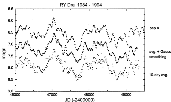
Figure 1. Comparison between the photoelectric and visual observations for RY Dra. See text for further explanation.
