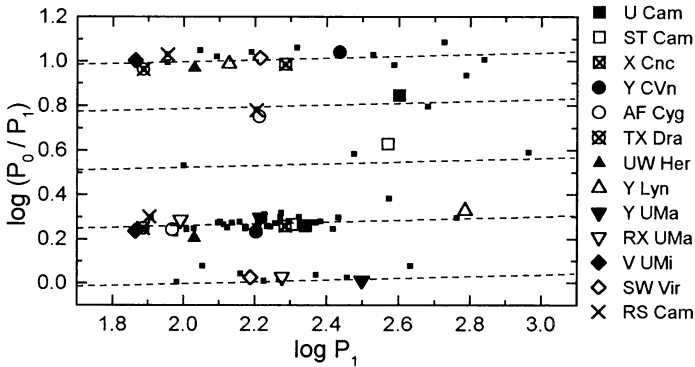
Figure 2. The Petersen diagram for all multiperiodic semiregulars. Triply periodic variables are plotted separately.
