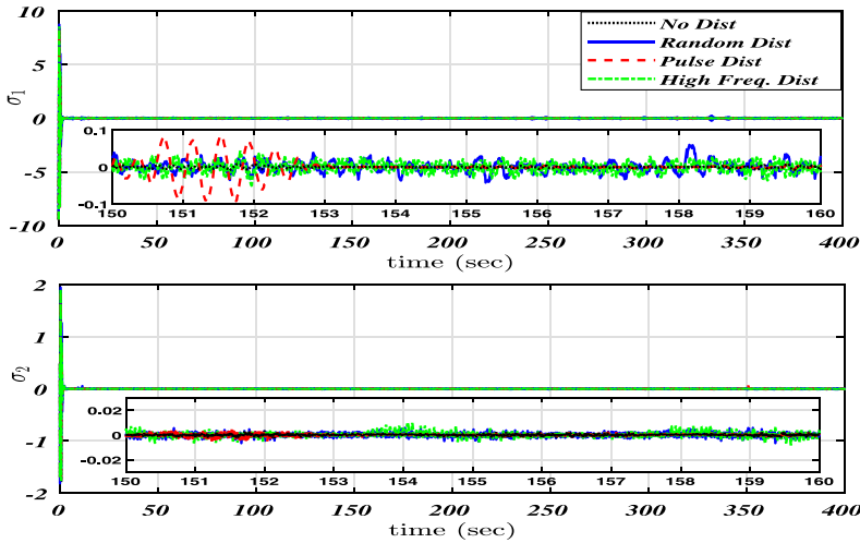
Figure 16. Sliding surface: sinusoidal path.
