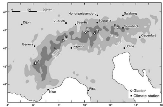
Fig. 2. Locations of glaciers and weather stations in the Alps with long records. A: Glacier de Sarnnes and Glacier de Saint-Sorlin; B: Griesgletscher; C: Silvrettagletscher; D: Hintereisferner, Kesselwandferner and Vernagtferner; E: Sonnblickkees.
