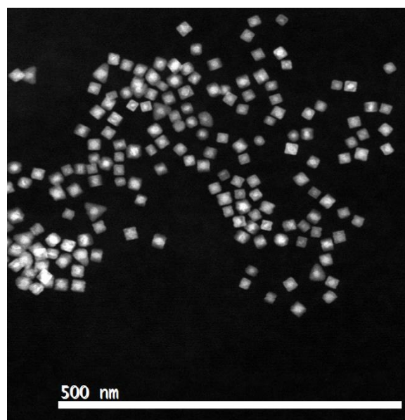
Figure 1: Ex situ HAADF STEM micrograph of Au-Pd core-shell nanocube as seen in S/TEM grid. The Z-contrast imaging showed that the nanocube is ~20 nm in size with the core made from Au (higher atomic number) and the shell made from Pd (lower atomic number).
