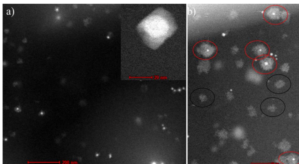
Figure 2: Low magnification in-situ STEM imaging of the formation of Au-Pd core-shell nanostructures from octahedral Au NPs. (a) Low magnification image shows that core-shell nanostructures are obtained with Au inside (core) and Pd outside (shell). A random area in Figure (a) is zoomed in and is presented in Figure (b) where the core-shell structure is clearly seen (represented by red circled regions). The core-shell ex-situ nanocubes are relatively smaller in size ~20 nm, while the in-situ (red circled) are larger in size ~60 nm. Some of the Pd nanocrystals were seen (represented by black black circles). Size controlled AuPd core-shell nanocube obtained from another static in situ experiment by changing the concentration of Pd precursor is inset in Fig. 2a, which shows the nanocube is made from Au core and some finite layer of Pd shell, indicating that the in situ experiment is close agreement with the ex situ experiments.
