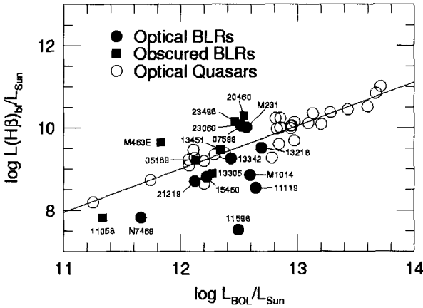
Figure 3. Dominant energy source of ultraluminous infrared galaxies based on their broad-line luminosities. The solid line is the best fit for the optical quasars. From Veilleux et al. (1999b).
