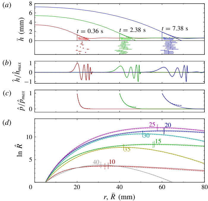
FIGURE 4. (Colour online) Results of the linear stability analysis for the D56/H56 latex cell with Q = 400 \text{ ml min}^{-1} . (a) Instantaneous base-state profiles \hat{h} (solid curves), and the corresponding approximate wedge profiles (dashed curves) at t = 0.36 , 2.38 and 7.38 s, respectively. The solid vertical lines indicate the position of the interface, and points with the horizontal error bars below indicate the position \bar{R} \pm \hat{R} observed in each of the 12 experiments. (b,c) The perturbations to the height and pressure profiles for a wavenumber n = 25 , normalized by the maximum absolute value. In (b), the dotted curves show the results from the ‘frozen-time’ approximation. In (c), \hat{p} is only plotted in the range r > \bar{R} , and the dashed curves show the profiles from the rigid-wedge approximation. (d) The evolution of amplitudes \hat{R} for a range of different wavenumbers, comparing the results from the full analysis (solid curves) to those obtained when using the rigid-wedge approximation (dashed curves). The maximum for each wavenumber is marked by a vertical bar.
