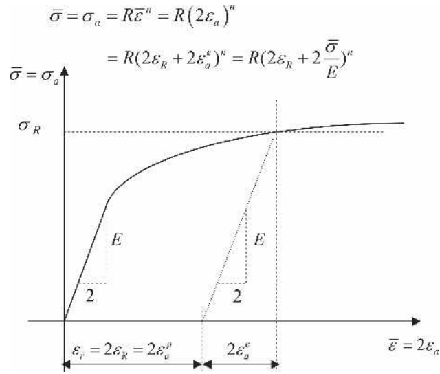
FIG. 1. Definition of the representative strain \epsilon_R and the representative stress \sigma_R(\epsilon_R) on the biaxial stress-strain curve, which is used in Refs. 1 and 2.
