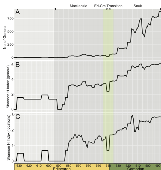
Figure 5. Time series of raw genus counts and the Shannon H indices of unique genus names and their reported locations (“states” field in the Paleobiology Database [PBDB]) with Mackenzie and Sauk Sloss sequences and the Ediacaran/Cambrian transition highlighted. A, Raw genus counts; B, Shannon H index of unique genera names and their occurrence frequencies; and C, Shannon H index of unique state names and their occurrence frequencies. Decreases in Shannon H indices from ca. 565–555 Ma and ca. 515–505 Ma represent intervals in which sampling is dominated by collections at specific localities (Mistaken Point Fm., Newfoundland, Canada, and Stephen Fm., British Columbia, Canada, respectively).
