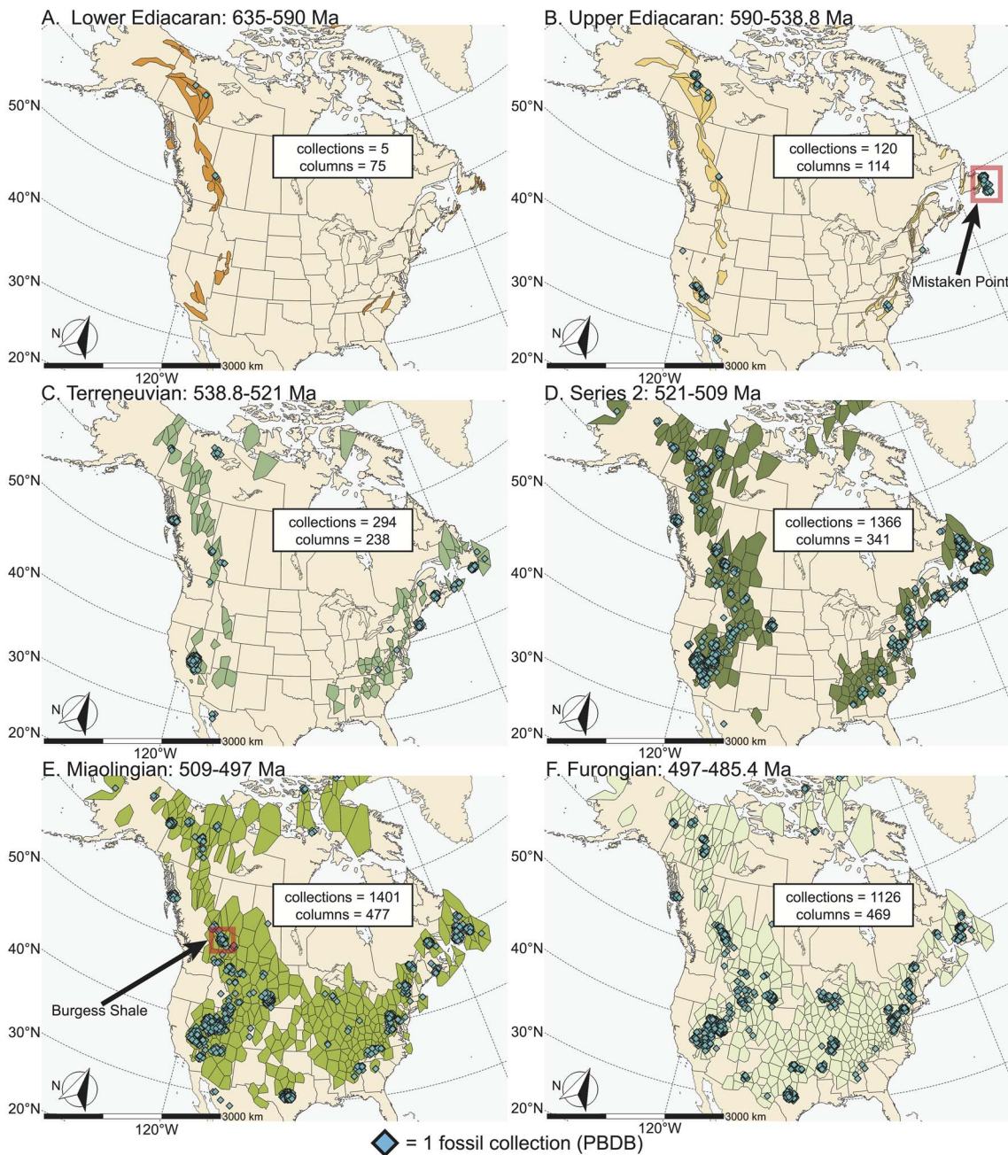
Figure 1. Maps of North America with sediment-bearing column areas from Macrostrat (colored polygons) and fossil collection locations from the Paleobiology Database (PBDB; blue diamonds). Fossil collection locations have been randomly offset by a factor of 0.5%. Total numbers of columns and fossil collections are shown on each map. A, Lower Ediacaran (635–590 Ma); B, upper Ediacaran (590–538.8 Ma); C, Terreneuvian (538.8–521 Ma); D, Series 2 (521–509 Ma); E, Miaolingian (509–497 Ma); F, Furongian (497–485.4 Ma). Lower Ediacaran and upper Ediacaran informal divisions based on initial rise in preserved sediment area and volume. Cambrian epoch timings based on Cohen et al. (2013; updated v2022/10).
