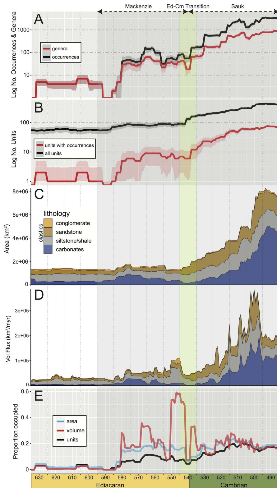
Figure 2. Time series of rock and fossil metrics from the Ediacaran and Cambrian with Mackenzie and Sauk Sloss sequences and the Ediacaran/Cambrian transition highlighted. A, Log-scale plot of the number of occurrences and genera with bootstrap resampling-generated confidence intervals ( 2\sigma ); B, log-scale plot of the total number of sedimentary rock units and the number of rock units that contain at least one fossil occurrence with bootstrap resampling-generated confidence intervals ( 2\sigma ); C, stacked area plot of preserved marine sedimentary rock area ( \text{km}^2 ) divided into clastic (grain size-based) and carbonate categories; D, stacked area plot of calculated marine sedimentary volume flux ( \text{km}^3/\text{Myr} ); and E, proportion of fossil-occupied sedimentary units (black), area (blue), and volume flux (red). Note that pre-580 Ma occurrences include fossil data from thicker, undivided stratigraphic sections with few geochronologic constraints.
