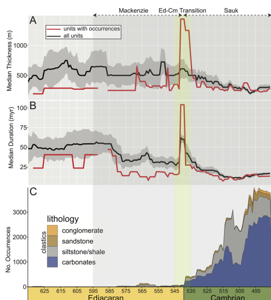
Figure 3. Time series of median thickness and duration of sedimentary rocks and the number of occurrences reported from clastic and carbonate lithologies with Mackenzie and Sauk Sloss sequences and the Ediacaran/Cambrian transition highlighted. A, Median thickness (m) of all sedimentary units (black) with bootstrap resampling-generated confidence interval ( 2\sigma ) and only sedimentary units that are occupied (contain at least one occurrence; red); B, median duration (Myr) of all sedimentary units (black) with bootstrap resampling-generated confidence interval ( 2\sigma ) and only sedimentary units that are occupied (red); and C, stacked area of occurrence counts by Paleobiology Database (PBDB) reported lithology. A single occurrence can have multiple lithologies and therefore can be counted within multiple lithologic categories for one time interval.
