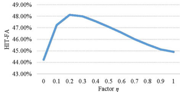
Fig. 3. Average HIT-FA score histogram with respect to factor \eta .
