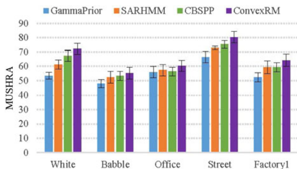
Fig. 10. The MUSHRA results for five types of noises.
