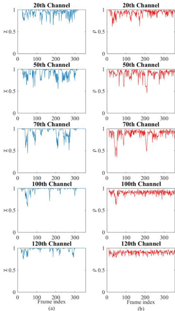
Fig. 5. An example of normalized cross-correlation coefficient in different channels (Input SNR = 5 dB, white noise). (a) True noise condition. (b) Estimated noise condition.
